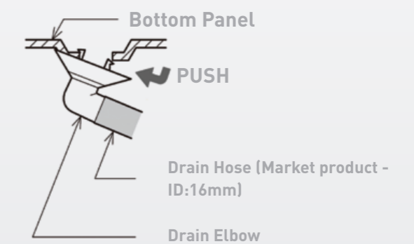
Figure 7: How to attach drain elbow.
