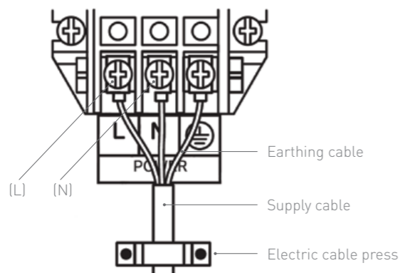
Figure 12: How to attach the power cable.
